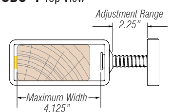
SBC-4 Top View
