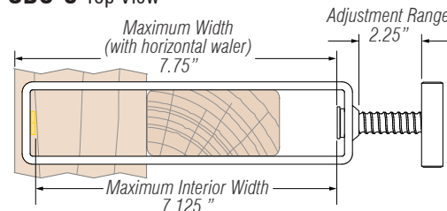
SBC-8 Top View
